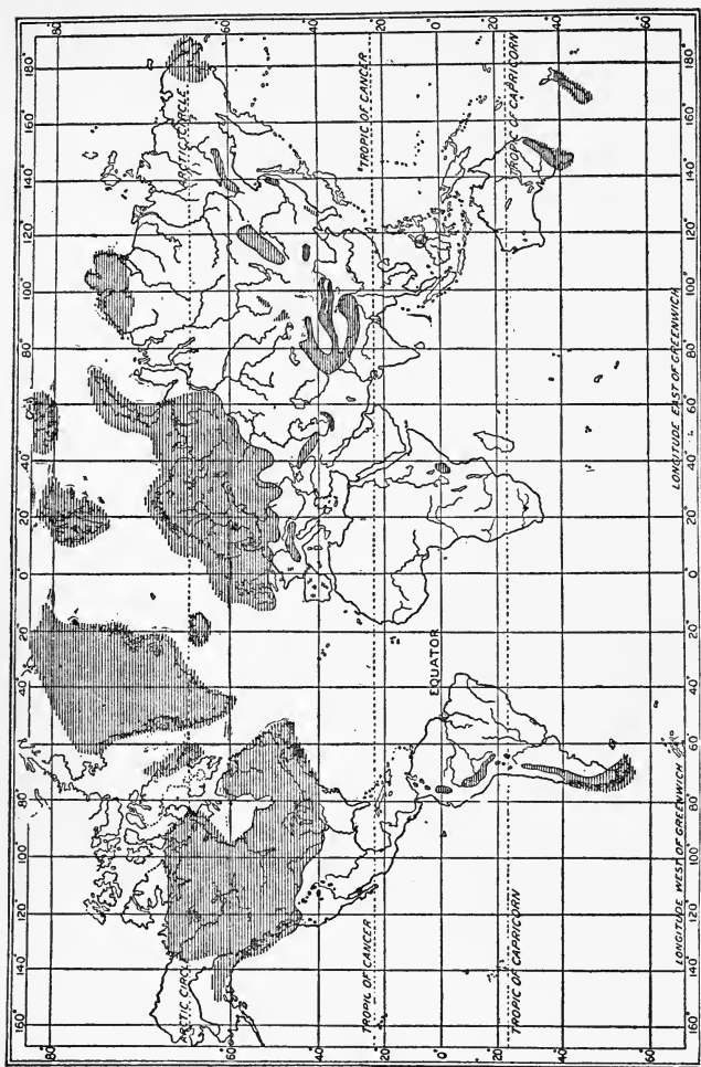
Fig. 6. Distribution of Pleistocene ice sheets.
